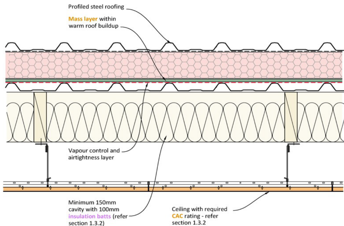
Figure 13: General design of approved warm roof solution
