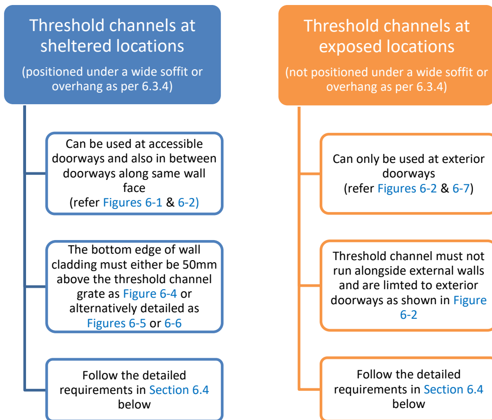
Figure 6-3 Summary Chart for Threshold Channel Usage
