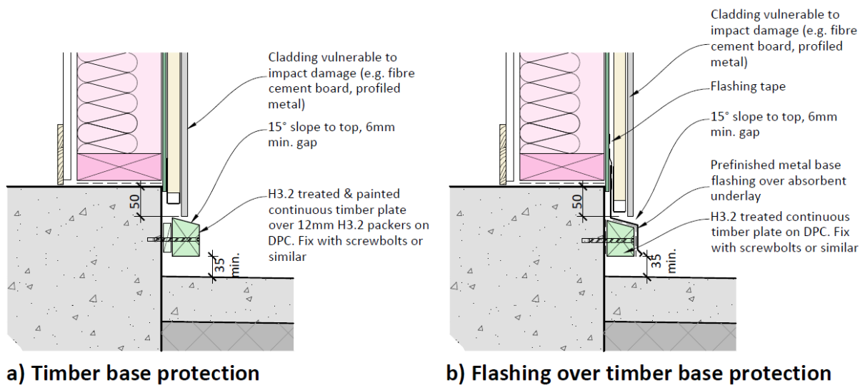
Figure 9-1 Cladding Base Protection Options
