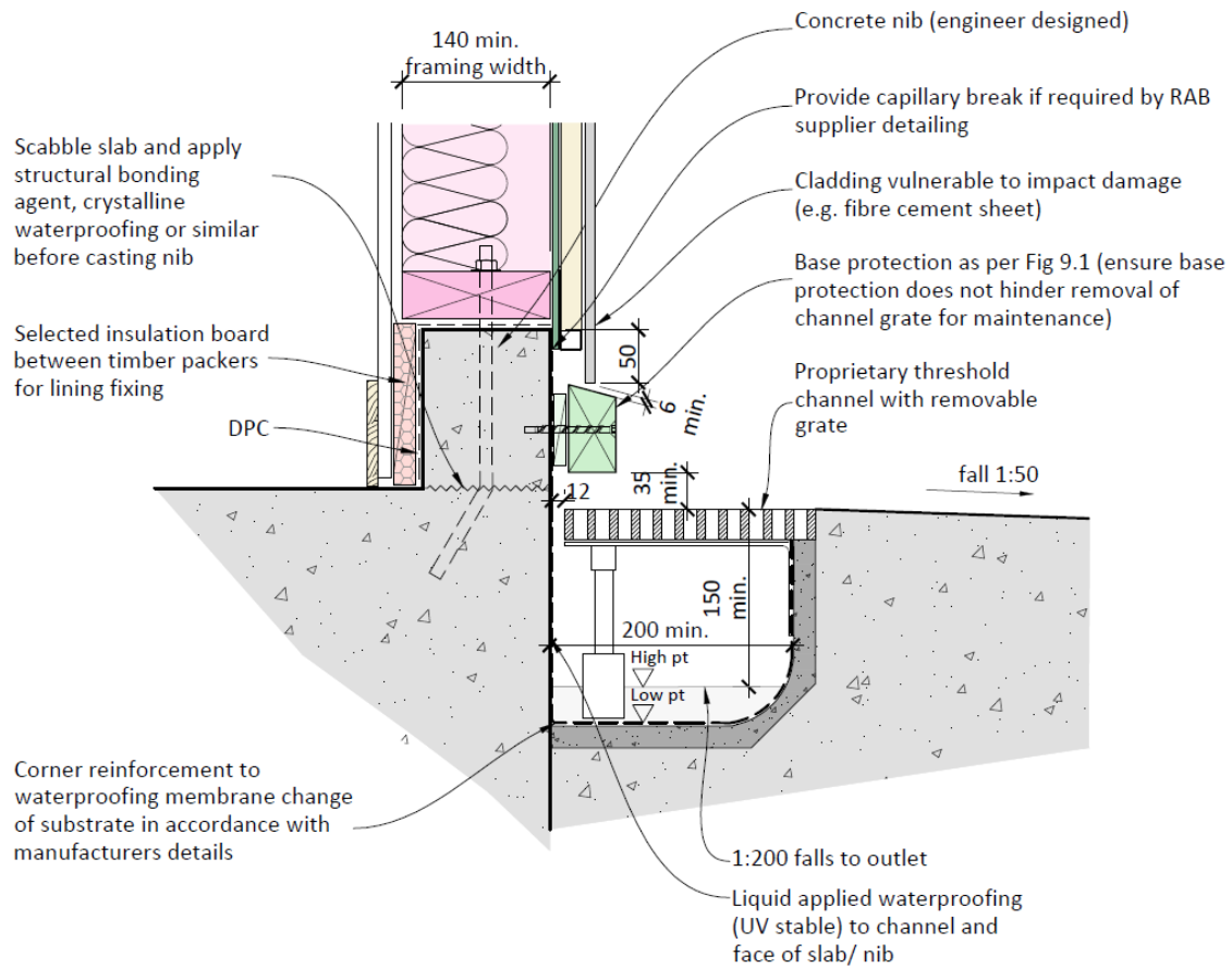
Figure 6-5 Threshold Channel to Cladding (with Cladding Base Protection)
