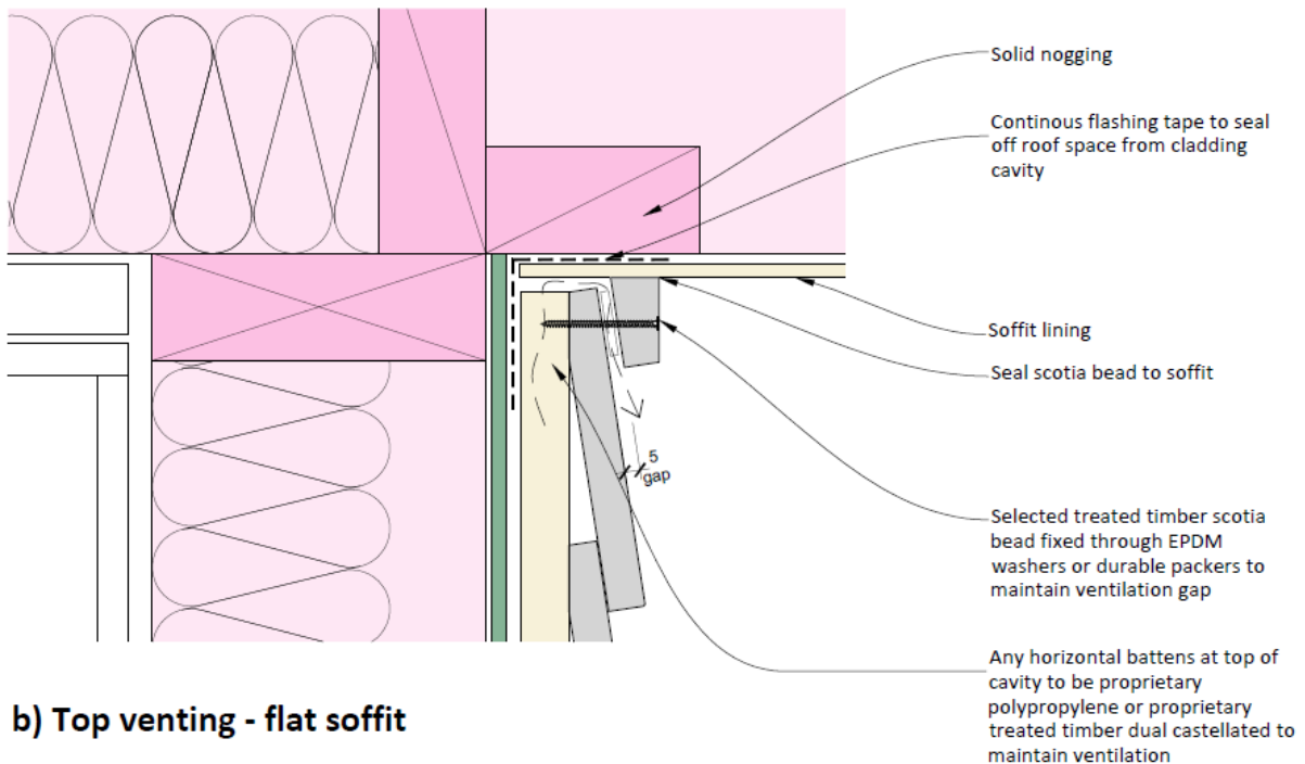
Figure 9-3 Top Venting
