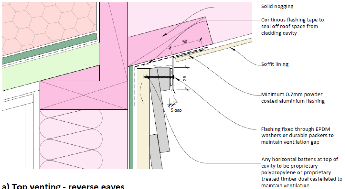
a) Top venting - reverse eaves
