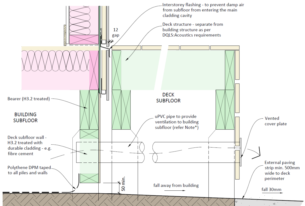
Figure 7-1 Sub-floor Wall between Deck and Building
