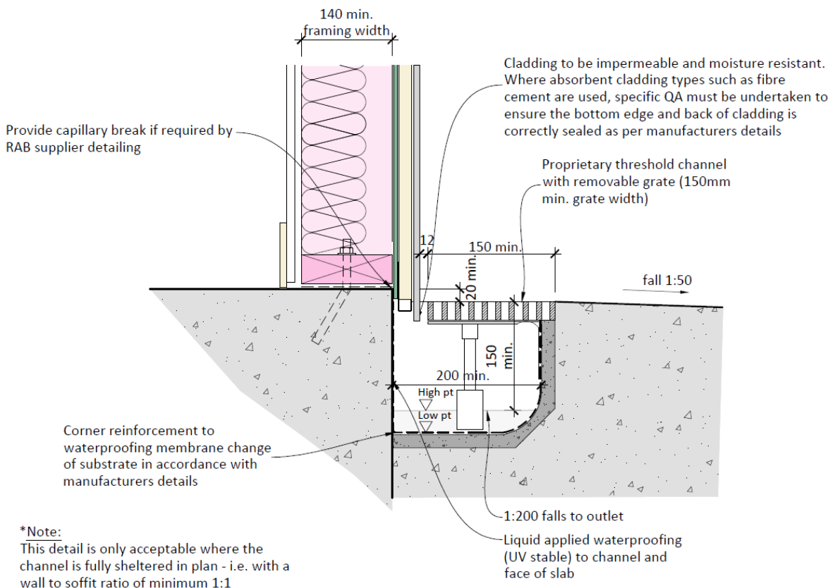
Figure 6-6 Threshold Channel to Cladding (alternative detail for sheltered locations)
